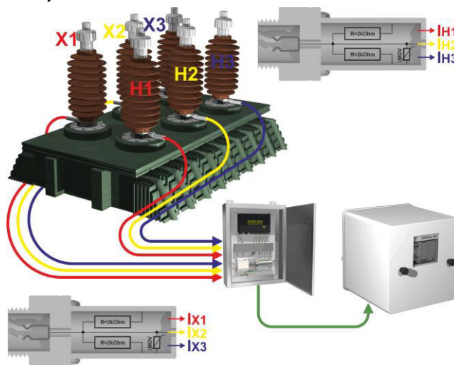
Monitoring of high- and low voltage side
